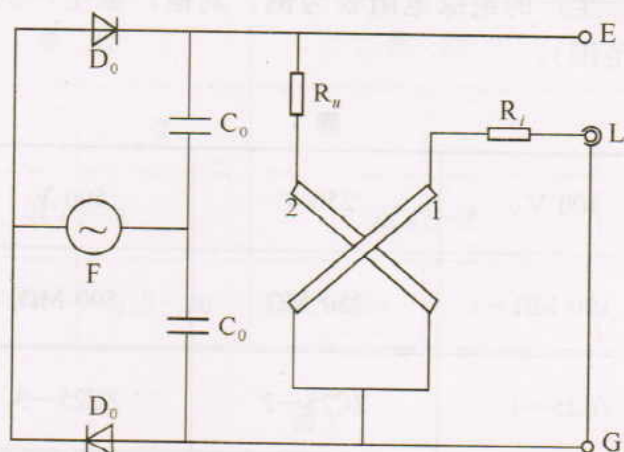
绝缘电阻表原理图
